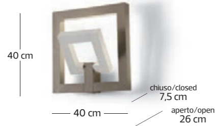
art. Ri_quadro A40-2 LED 3510 LM 32 W 3000 K
