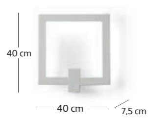
art. Ri_quadro A40 LED 2250 LM 20 W 3000 K
