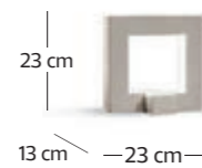
art. Ri_quadro LP LED 1260 LM 12 W 3000 K
